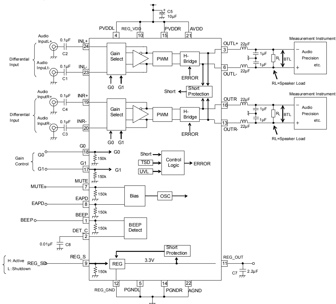
Evaluation Circuit Diagram
