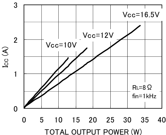
Fig. 10 Current consumption - Output power
