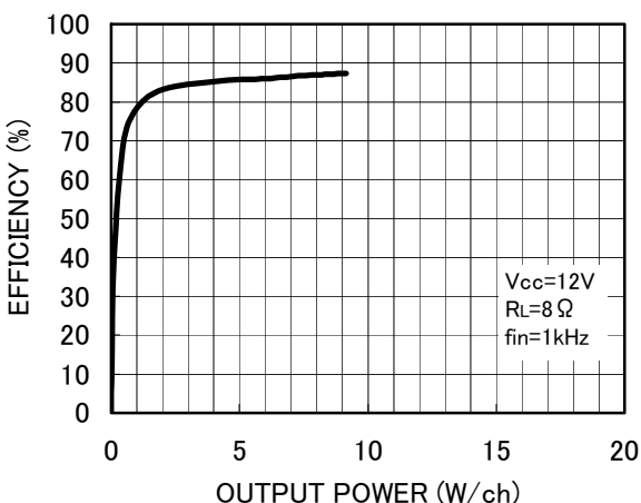
Fig. 8 Efficiency - Output power
