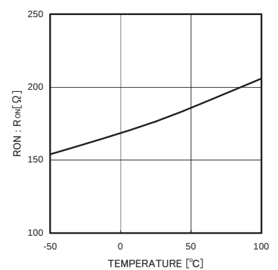
Fig11. ON Resistance
