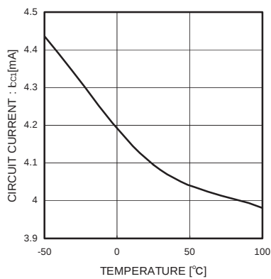
Fig3. Circuit Current1
