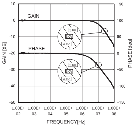
Fig5. Frequency characteristics (Supply voltage dependence)
