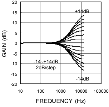
Fig.12 Treble Gain - Frequency
