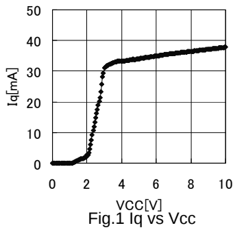
Fig.1 I_q vs V_{CC}
