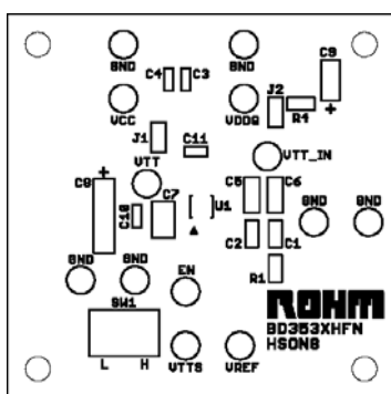
Silk Screen
