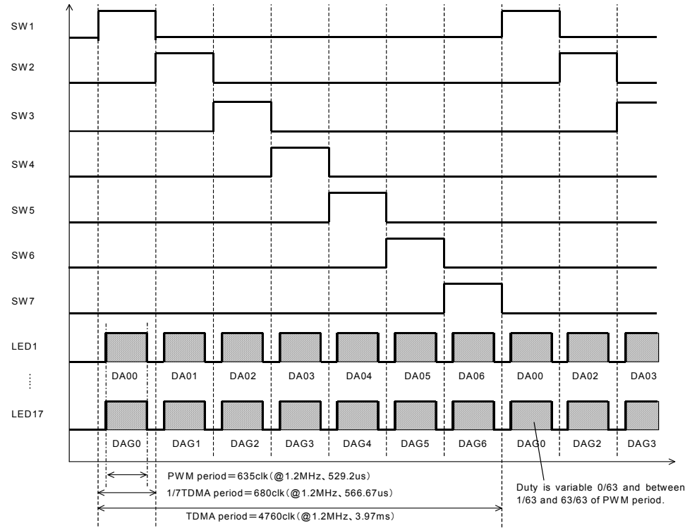
Fig.11 SW timing
