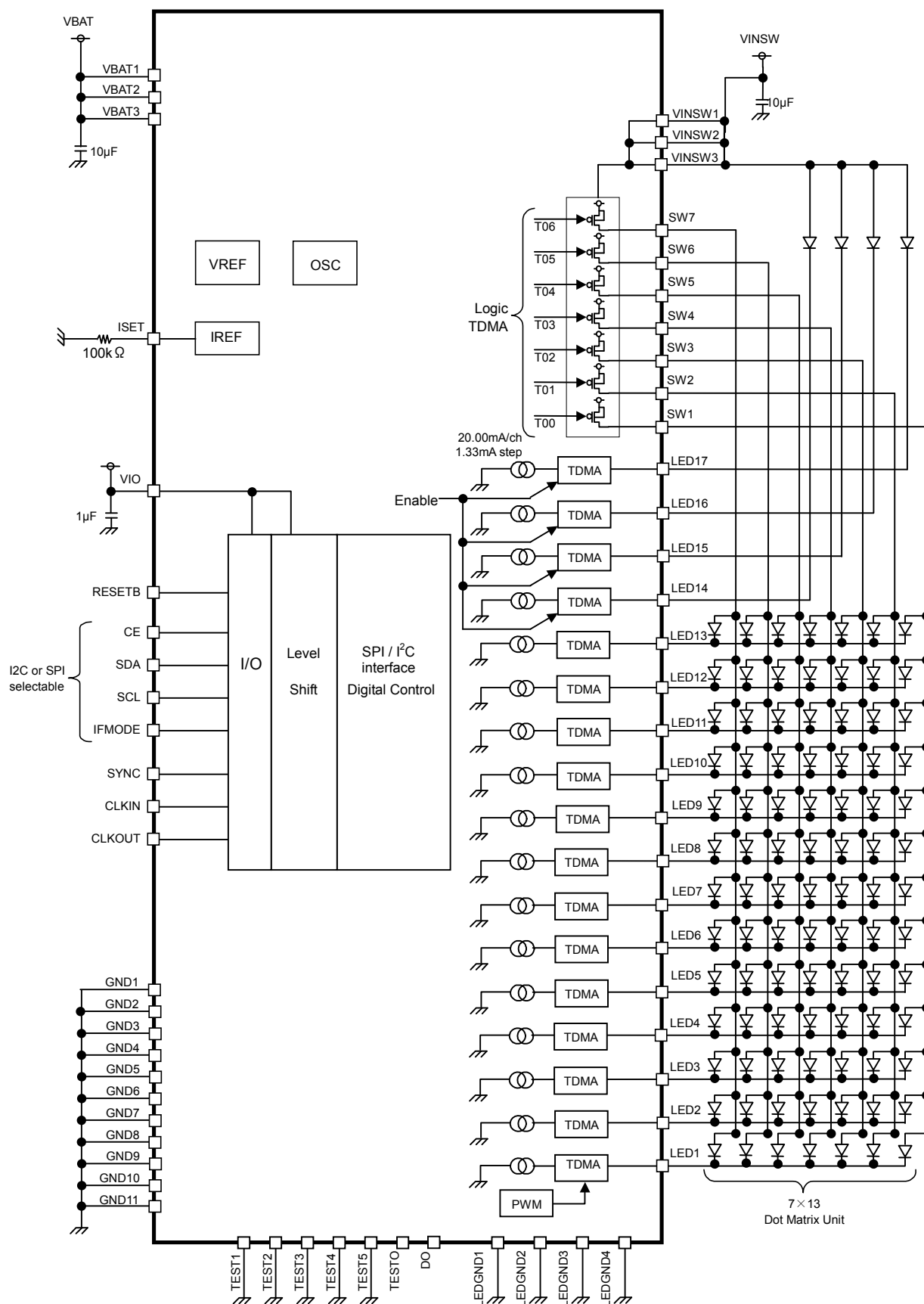
Fig.3 Block Diagram / Application Circuit example 2
