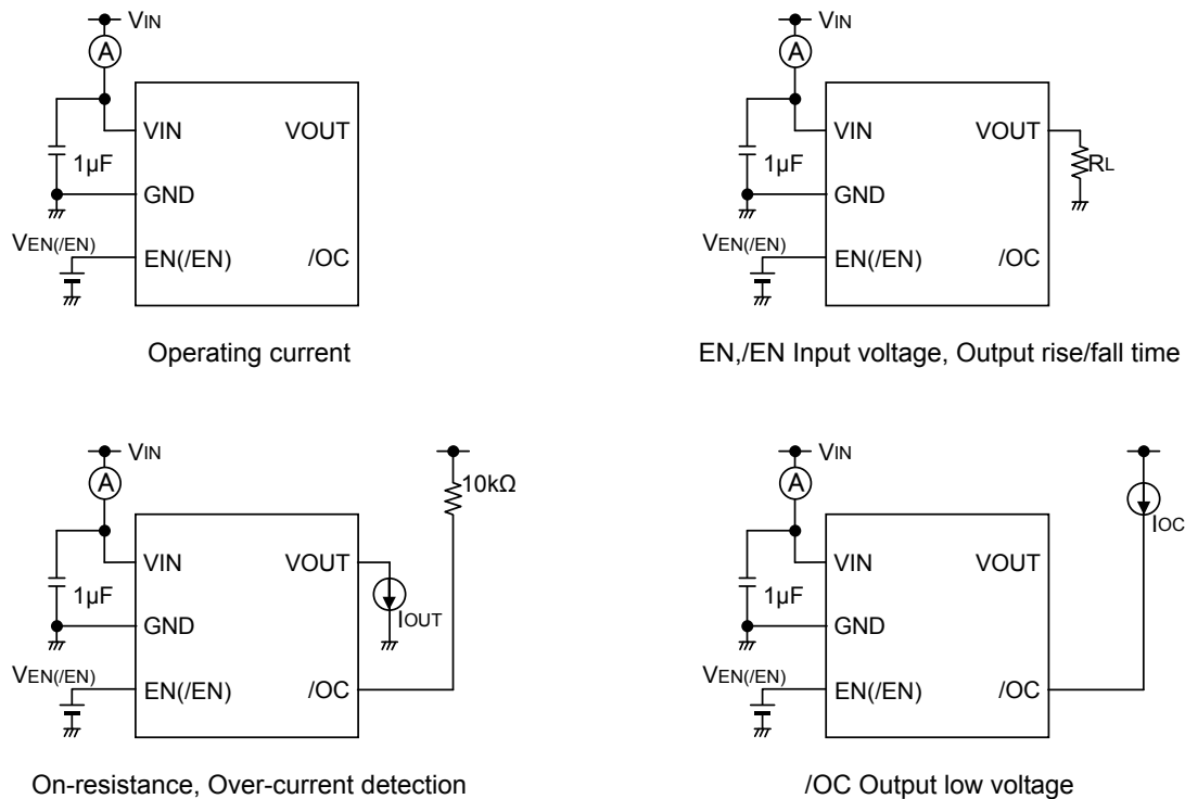
Fig.1 Measurement circuit
