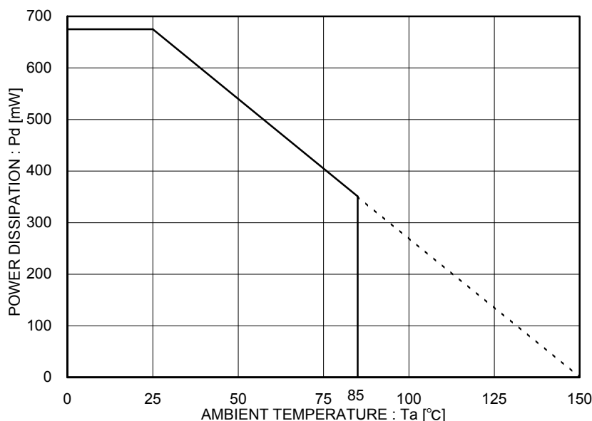
Fig.45 Power Dissipation Curve (Pd-Ta Curve)
