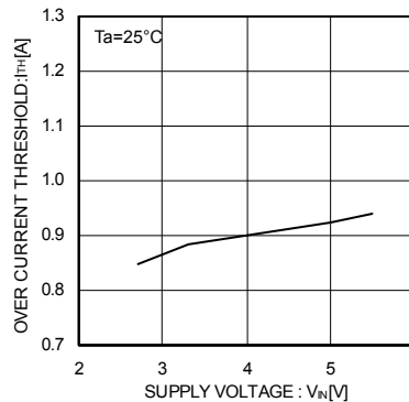
Fig.12 Over-current threshold
