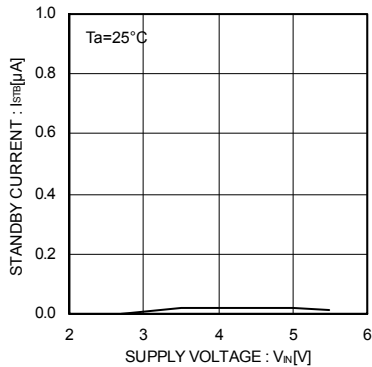
Fig.6 Standby current EN,/EN disable
