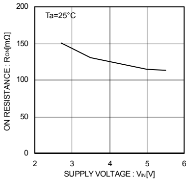
Fig.10 On-resistance
