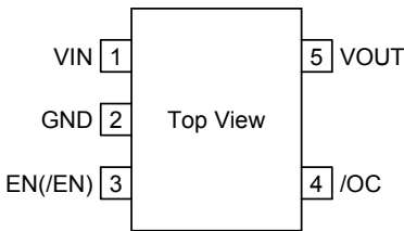
Fig.40 Pin configuration
