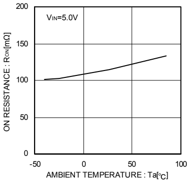
Fig.11 On-resistance
