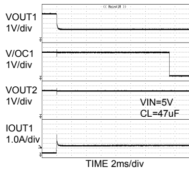
Fig.35 Over-current response 1 \Omega load connected at enable
