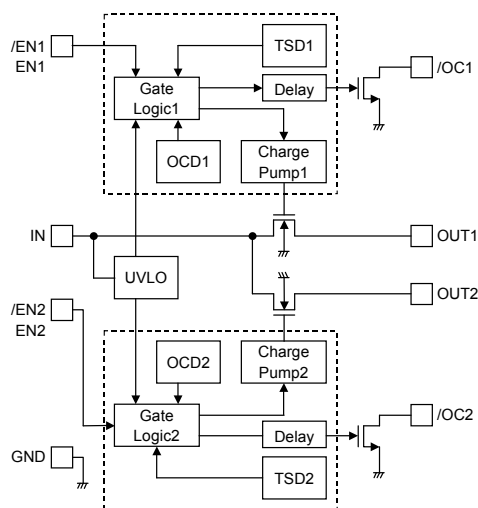
Fig.38 Block diagram
