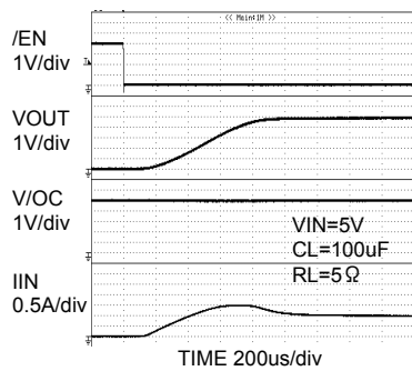
Fig.30 Output rise characteristics
