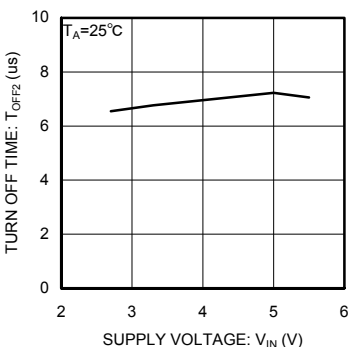
Fig.24 Output turn-off time
