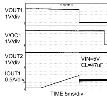
Fig.34 Over-current response ramped load
