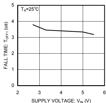
Fig.22 Output fall time
