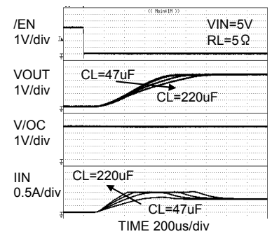
Fig.32 Inrush current \text{CL}=47\mu\text{F} , 100\mu\text{F} , 147\mu\text{F} , 220\mu\text{F}
