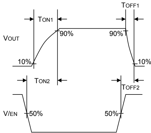
Fig.2 Timing diagram
