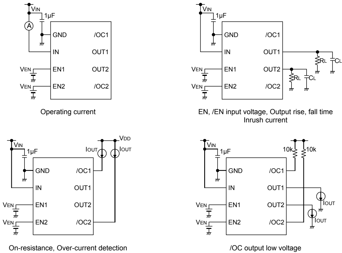
Fig.1 Measurement circuit
