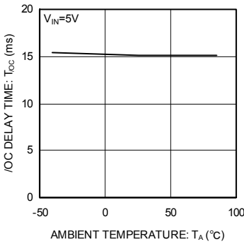
Fig.27 /OC delay time
