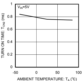
Fig.21 Output turn-on time
