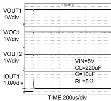
Fig.33 Inrush current
