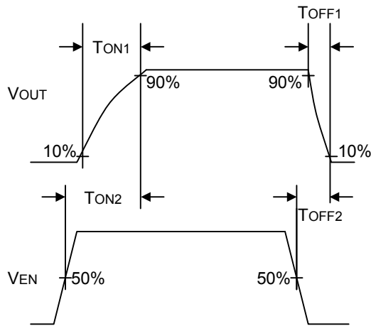
Fig.3 Timing diagram
