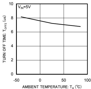
Fig.25 Output turn-off time
