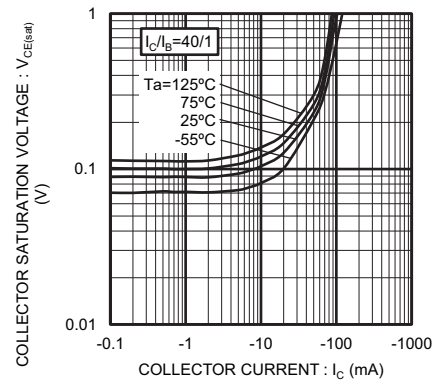
Fig6. Collector Saturation Voltage vs. Collector Current (II)
