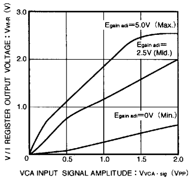
Fig. 18 V/I register output voltage vs VCA input signal amplitude
