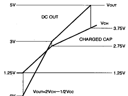
Fig. 22 Charging capacitor vs. DC output characteristic
