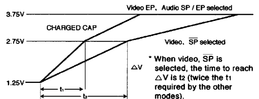
Fig.21 Charging capacitor voltage characteristic
