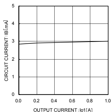
Fig. 2 Circuit Current vs Load Current I o2 (I o1 = 0 → 1 A)
