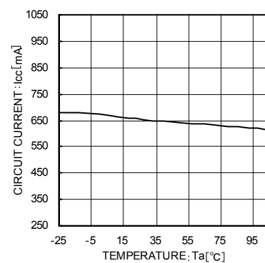
Fig. 24 Circuit Current vs Temperature (I o = 0 mA)
