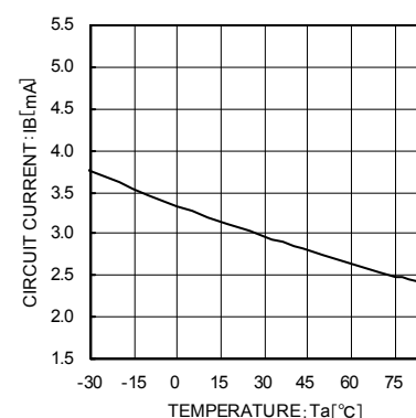
Fig. 12 Circuit Current vs Temperature (I o = 0 mA)
