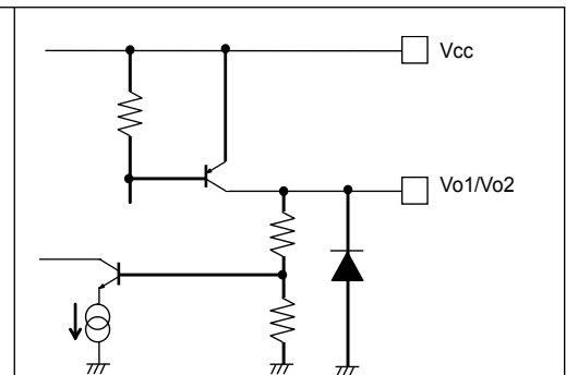
Fig. 28 BA33D□□Series Equivalent Circuit
