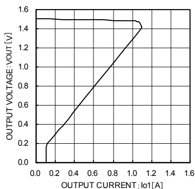
Fig. 19 Load Stability (1.5 V output)
