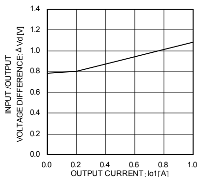
Fig. 8 I/O Voltage Difference (3.3 V output) ( V_{cc} = 3.8\text{V} , I o1 = 0 → 1 A)
