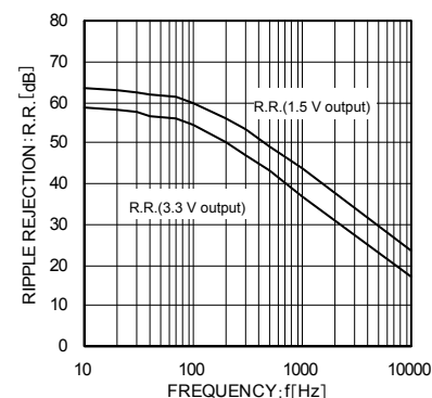
Fig. 9 R.R. Characteristics ( e_{in} = 0.5\text{Vp-p} , I o = 5 mA)
