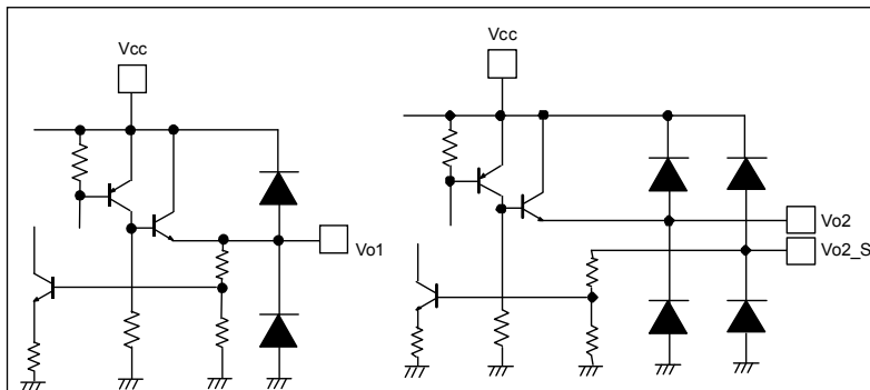
Fig. 27 BA3258HFP Input / Output Equivalent Circuit
