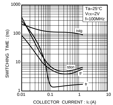
Fig.6 Switching time
