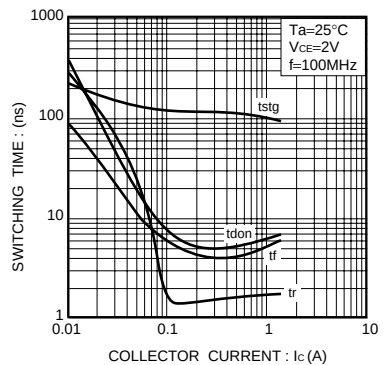
Fig.6 Switching time
