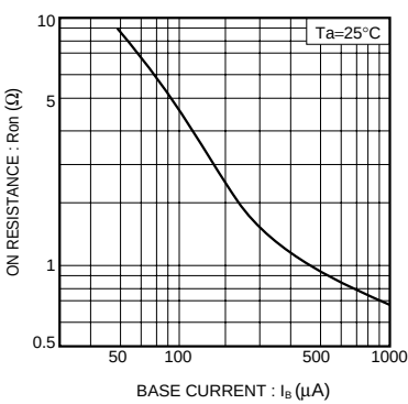
Fig.12 "ON" resistance vs. base current characteristics
