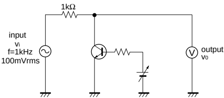
Fig.13 "ON" resistance measurement circuit
