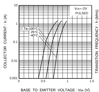
Fig.5 Grounded emitter propagation characteristics
