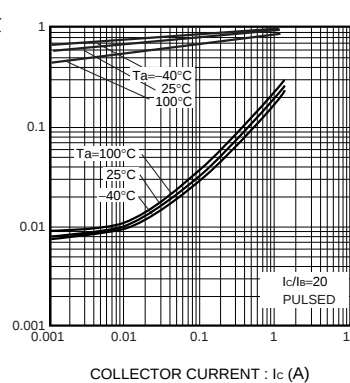
Fig.2 Collector-emitter saturation voltage vs. collector current Fig.3 Base-emitter saturation voltage vs. collector current
