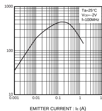
Fig.6 Gain bandwidth product vs. emitter current
