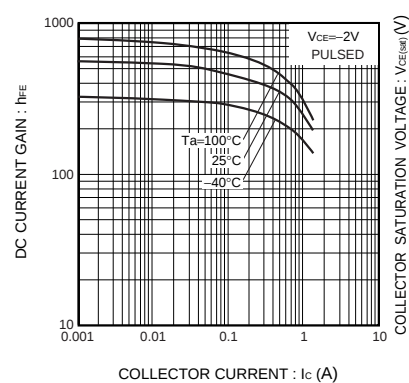
Fig.1 DC current gain vs. collector current
