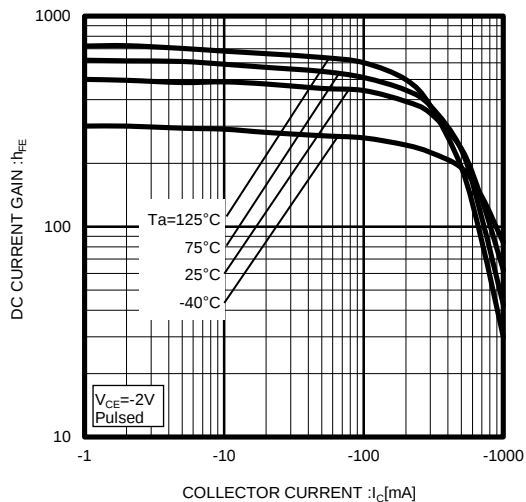
Fig.3 DC Current Gain vs. Collector Current( II )
