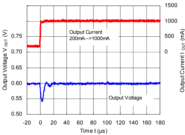
RP506Kxx1D/E/F ( V_{IN}=3.6V , V_{OUT}=0.6V )
