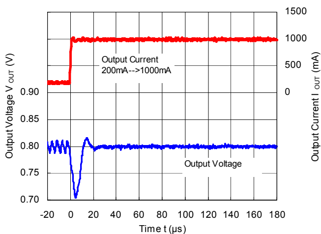
RP506Kxx1D/E/F ( V_{IN}=3.6V , V_{OUT}=0.8V ) MODE="H" Forced PWM Control
