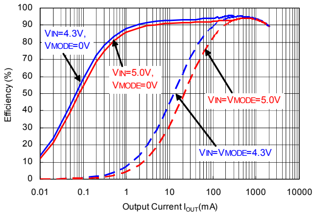
RP506Kxx1D/E/F V_{OUT}=0.6V
