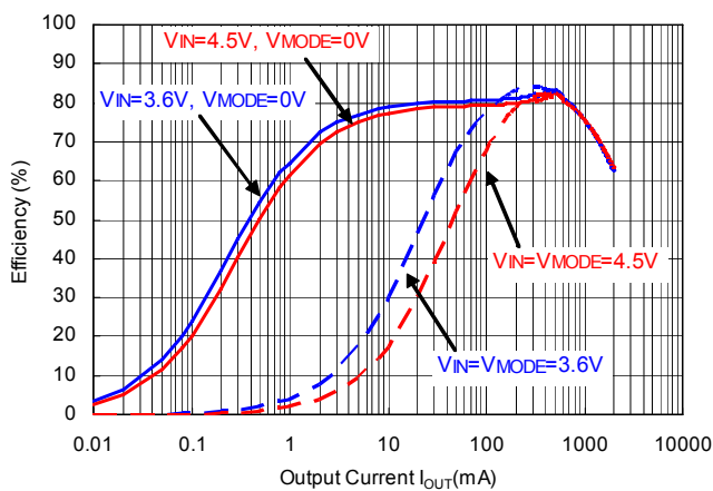
RP506Kxx1D/E/F V_{OUT}=0.6V
