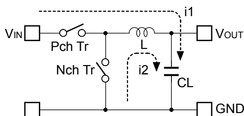
Diag. 1 Basic Circuit
