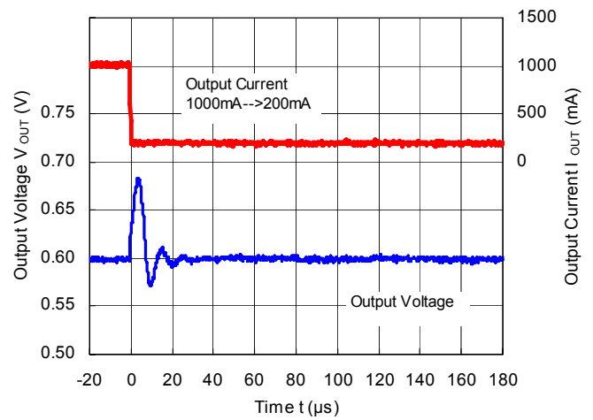
RP506Kxx1D/E/F ( V_{IN}=3.6V , V_{OUT}=0.6V )
