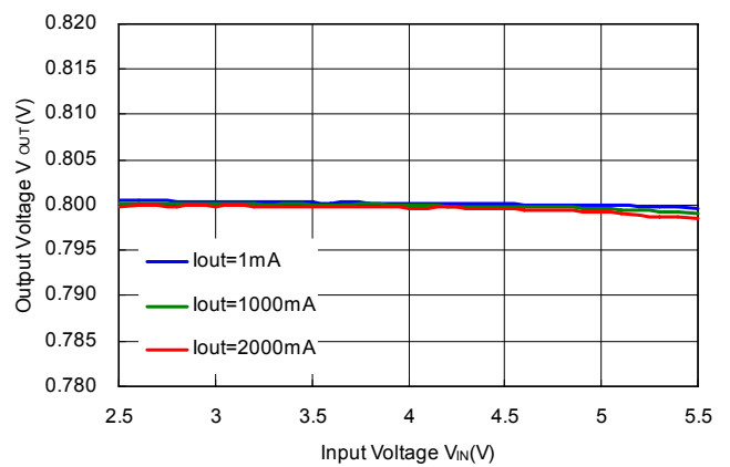
RP506Kxx1D/E/F V_{OUT}=0.8V
