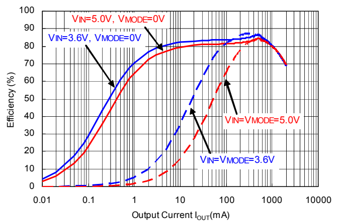
RP506Kxx1D/E/F V_{OUT}=0.8V
