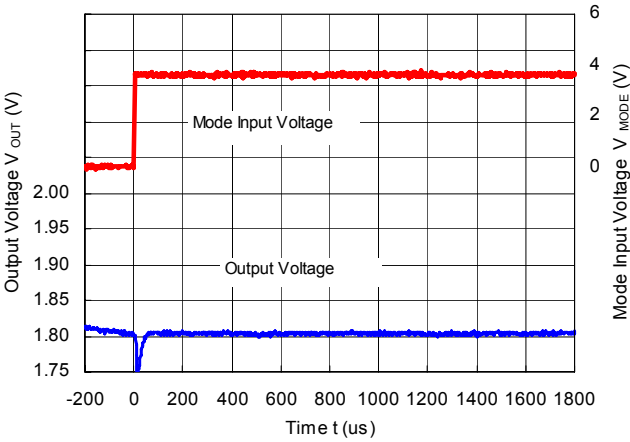
RP506Kxx1D/E/F ( V_{IN}=3.6V , V_{OUT}=1.8V , I_{OUT}=1mA ) MODE="L" --> MODE="H"
