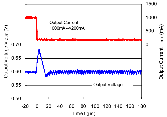
RP506Kxx1D/E/F ( V_{IN}=3.6V , V_{OUT}=0.6V ) MODE="H" Forced PWM Control
