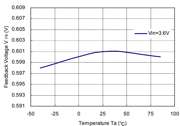
4) Feedback Voltage vs. Ambient Temperature RP506K001C/F
