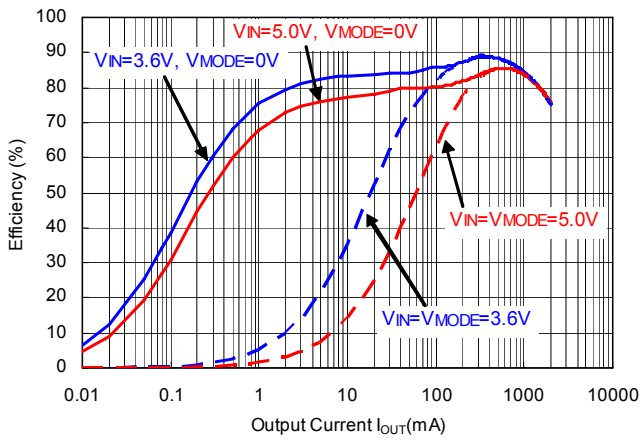
RP506Kxx1A/B/C V_{OUT}=3.3V
