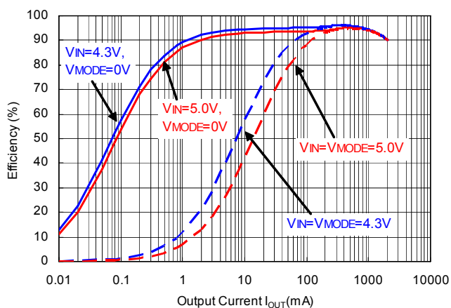
RP506Kxx1D/E/F V_{OUT}=3.3V
