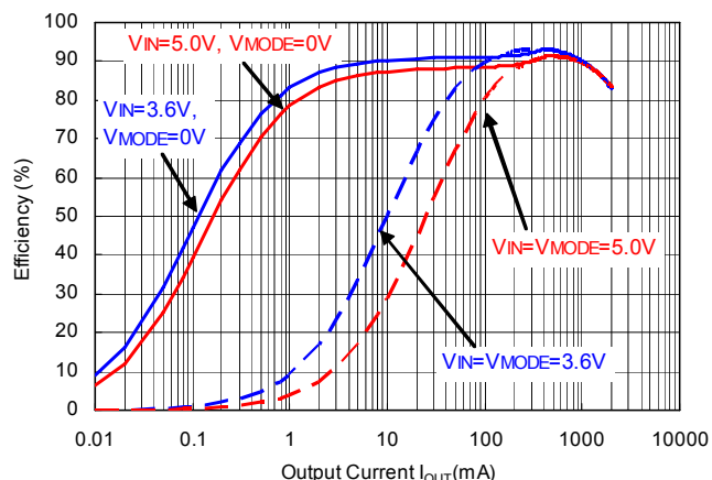
RP506Kxx1D/E/F V_{OUT}=1.8V
