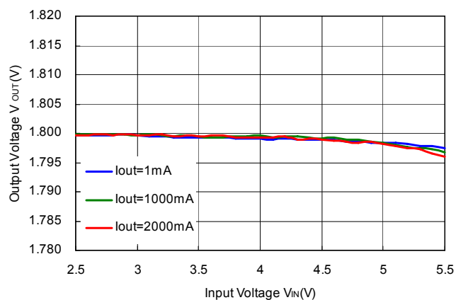
RP506K V_{OUT}=1.8V MODE="H" Forced PWM Control
