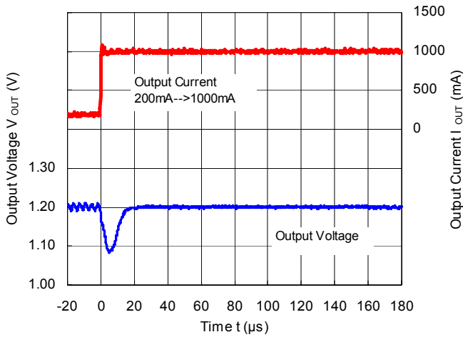
RP506Kxx1D/E/F ( V_{IN}=3.6V , V_{OUT}=1.2V ) MODE="H" Forced PWM Control
