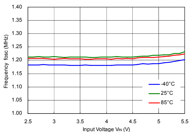
RP506Kxx1D/E/F
