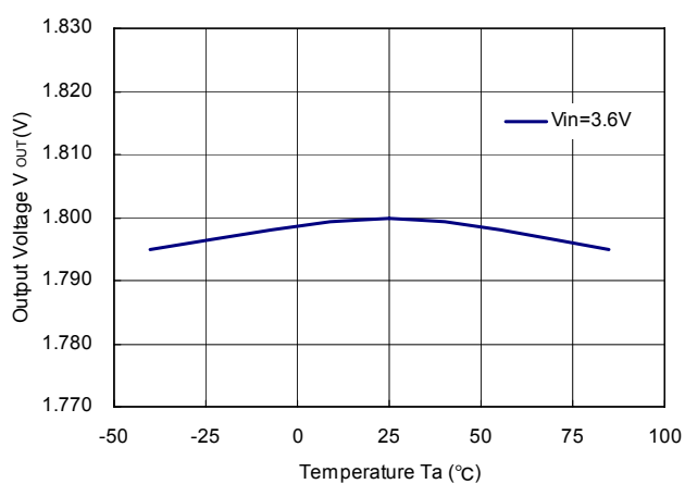
3) Output Voltage vs. Ambient Temperature RP506K181A/B/D/E V_{OUT}=1.8V
