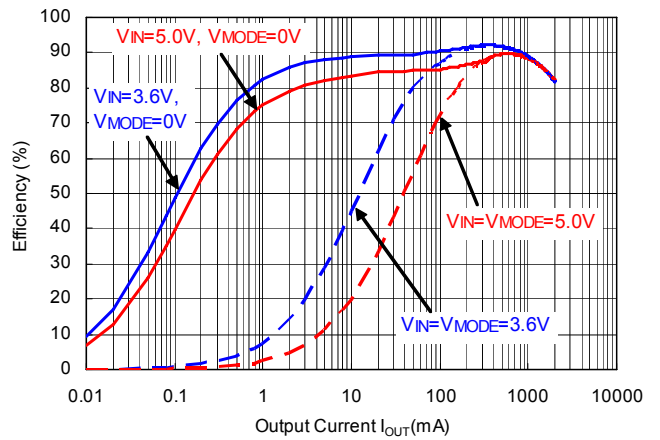
RP506Kxx1A/B/C V_{OUT}=1.8V
