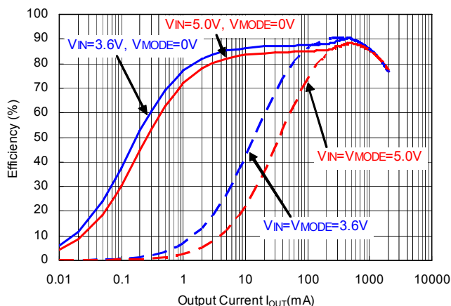
RP506Kxx1D/E/F V_{OUT}=3.3V
