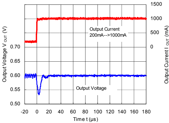
RP506Kxx1D/E/F ( V_{IN}=3.6V , V_{OUT}=0.6V ) MODE="H" Forced PWM Control
