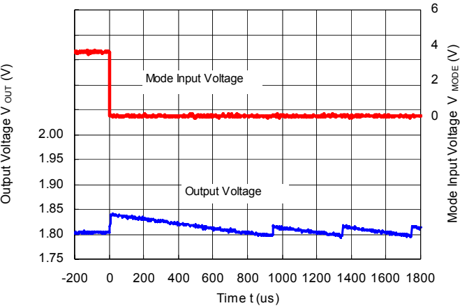
RP506Kxx1D/E/F ( V_{IN}=3.6V , V_{OUT}=1.8V , I_{OUT}=1mA ) MODE="H" --> MODE="L"
