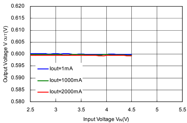
RP506Kxx1D/E/F V_{OUT}=0.6V
