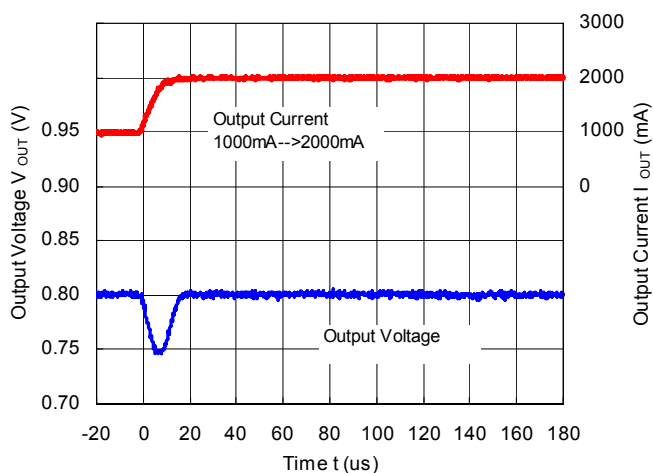
RP506Kxx1D/E/F ( V_{IN}=3.6V , V_{OUT}=0.8V )
