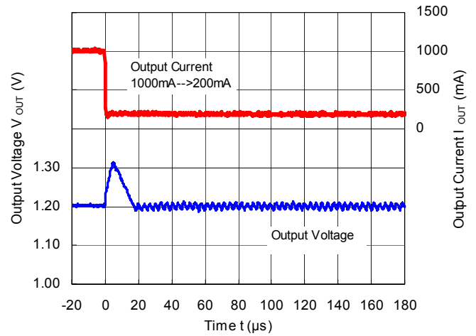
RP506Kxx1D/E/F ( V_{IN}=3.6V , V_{OUT}=1.2V ) MODE="H" Forced PWM Control
