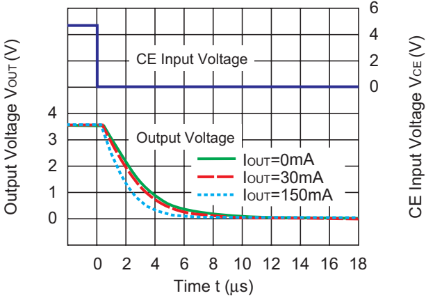
3.6V C Version (VR2) V_{IN}=4.6V
