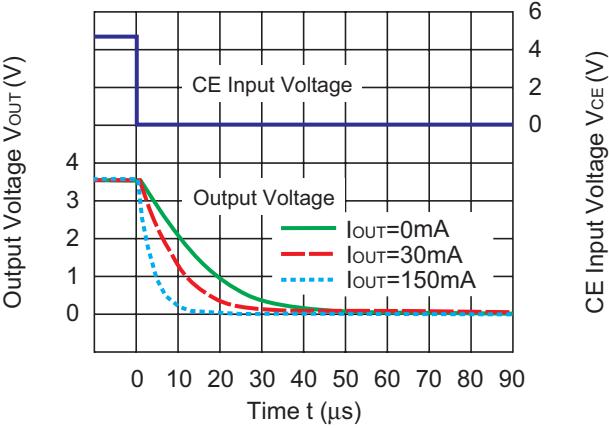
3.6V B Version (VR1/ VR2), C Version (VR1) V_{IN}=4.6V
