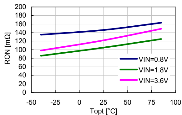
Switch On Resistance
