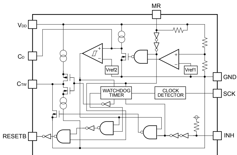
CMOS Output (R5107Gxx1C)
