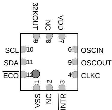
R2221L(QFN018018-12:underdevelopment)
