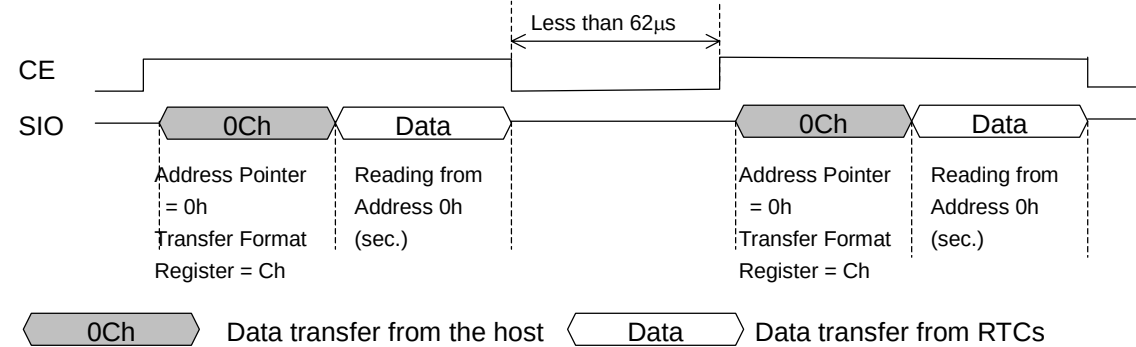
Bad Example (3) (Where a time span of less than 62µs is left between the adjacent processes of reading time data)
