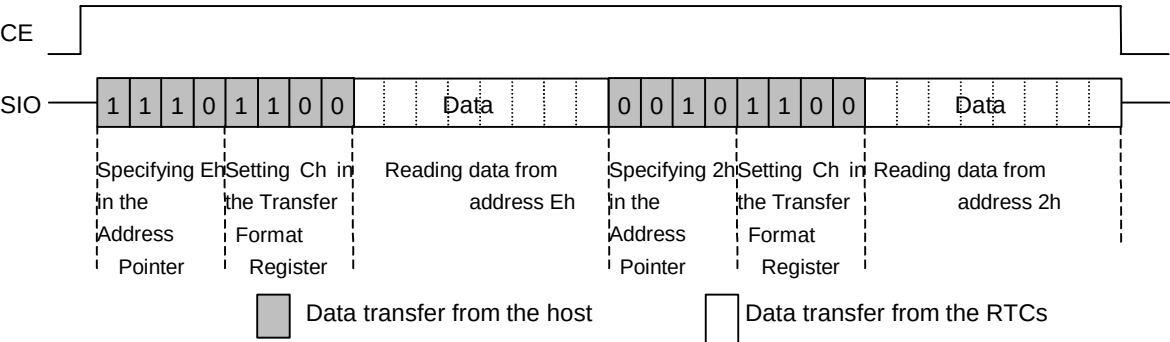
Example of 1-byte Reading Data Transfer (For Reading Data from Addresses Eh and 2h)
