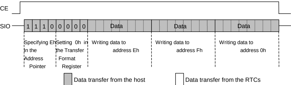
Example of Burst Writing Data Transfer (For Writing Data to Addresses Eh, Fh, and 0h)
