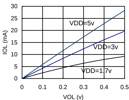
V_{OL} vs. I_{OL} (SCL pin) ( T_{opt}=25^{\circ}C )
