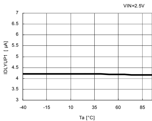
35) DELAY Charge Current VS. Temperature R1290K102A
