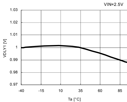
37) DELAY Detector Threshold VS. Temperature R1290K102A
