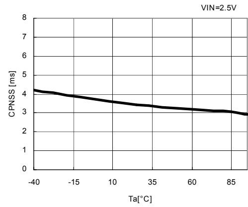
23) CPN Soft-Start VS. Temperature. R1290K102A
