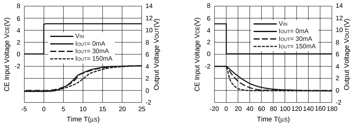
R1114x401D (V IN =5.0V, C IN =Ceramic 0.47μF, C OUT =Ceramic 0.47μF)
