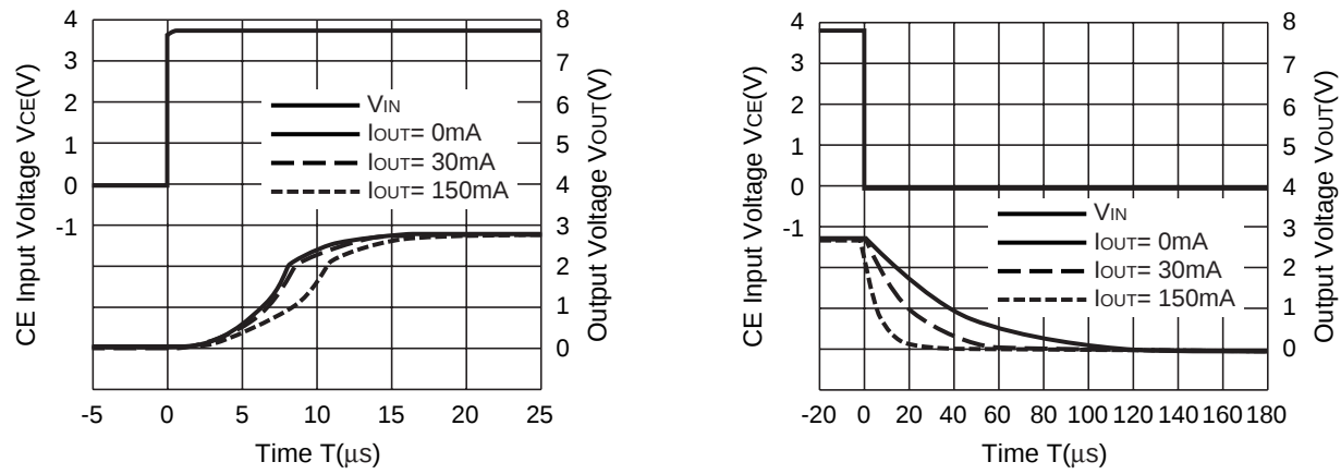
R1114x281D (V IN =3.8V, C IN =Ceramic 0.47μF, C OUT =Ceramic 0.47μF)
