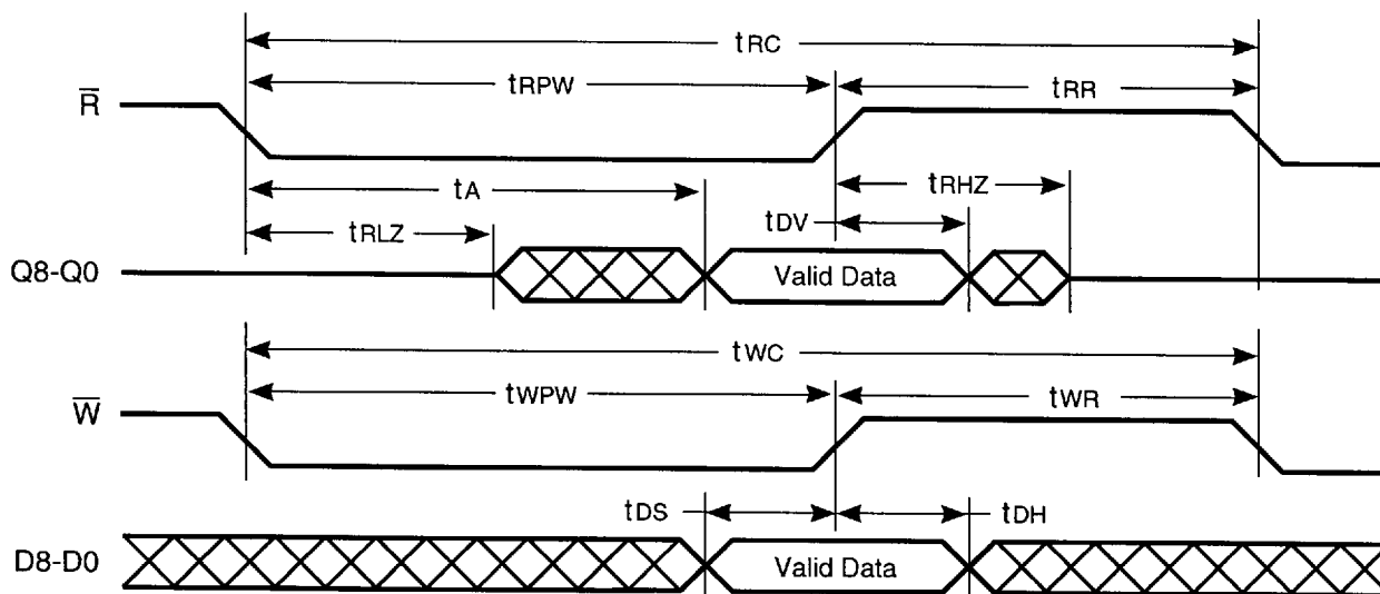
FIGURE 4. ASYNCHRONOUS READ AND WRITE OPERATIONS
