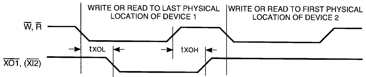
FIGURE 12. EXPANSION-OUT TIMING
