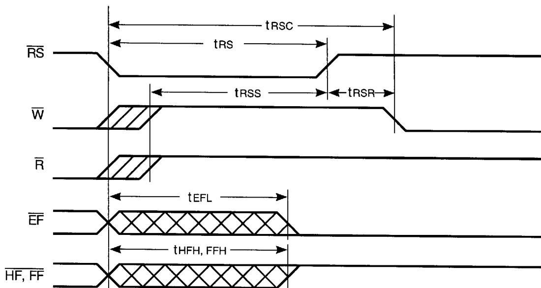
FIGURE 5. RESET TIMING
