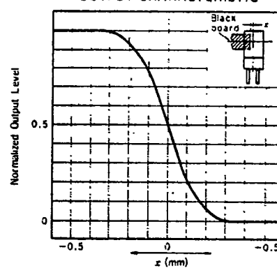
OUTPUT CHARACTERISTIC
