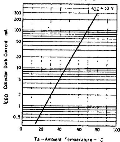
COLLECTOR DARK CURRENT vs. AMBIENT TEMPERATURE
