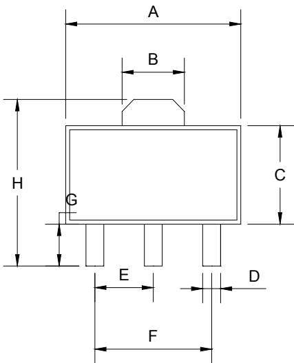
1.Top View
