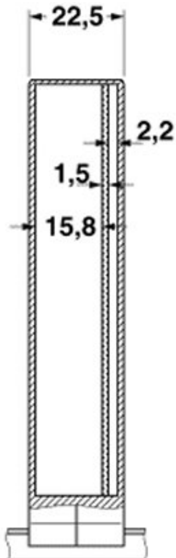
Dimensioned drawing
