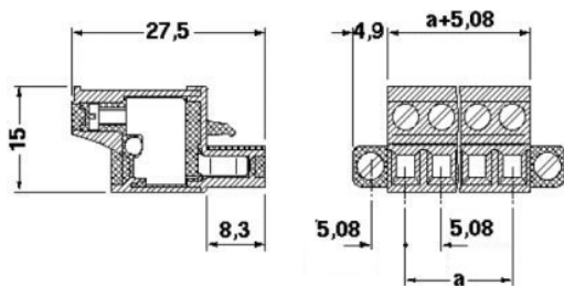
Dimensioned drawing
