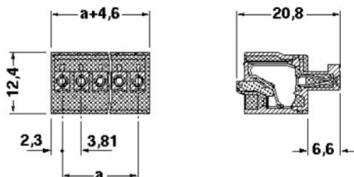
Dimensioned drawing
