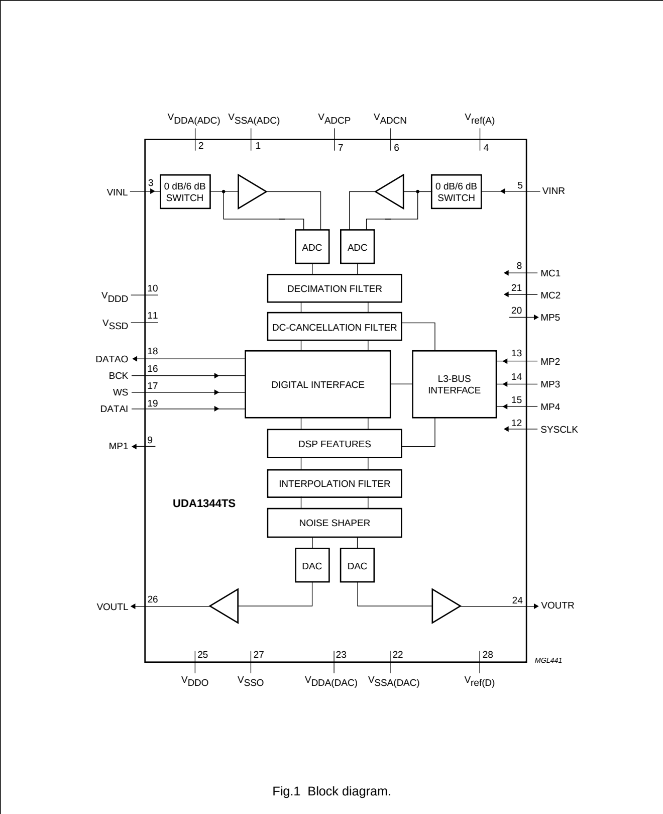
BLOCK DIAGRAM
