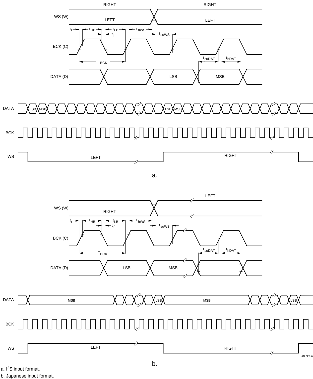
Fig.7 Timing diagram for the serial input and output formats.
