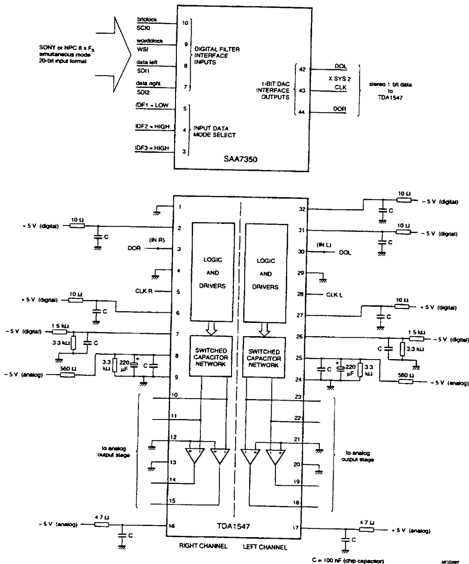
Fig.5 Application diagram.
