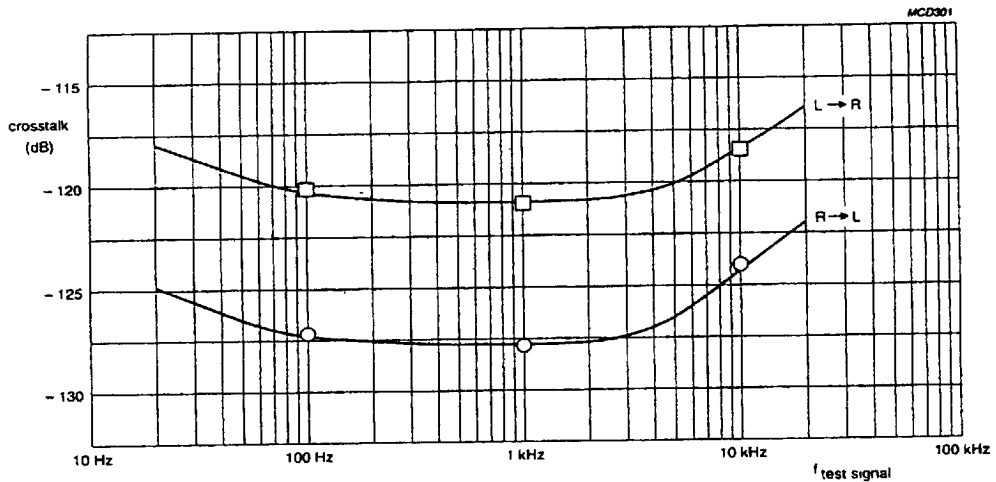
Fig.9 Inter-channel crosstalk as a function of signal frequency.
