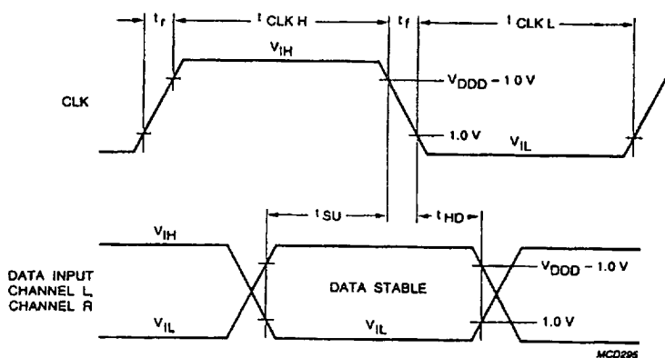
Fig.3 Timing waveform.
