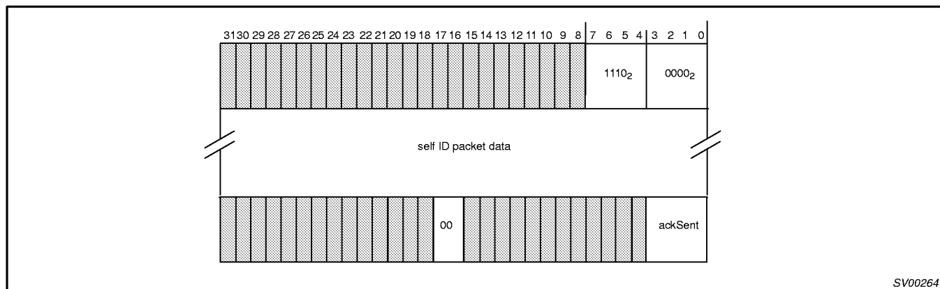
Figure 19. Self-ID Receive Format
