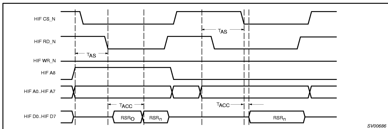
Figure 2. Read cycle signal timing (2 independent read cycles)
