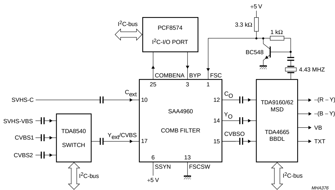
Fig.12 Application diagram: SAA4960 with TDA9160/62.
