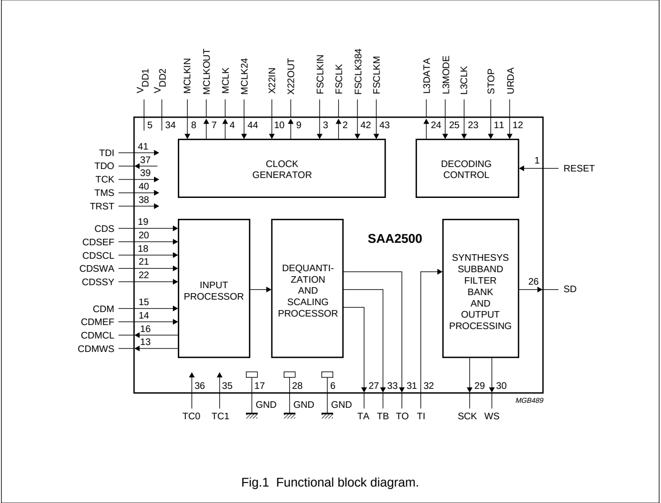
BLOCK DIAGRAM
