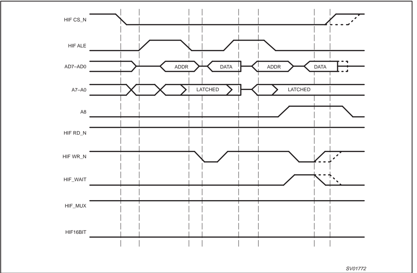
Figure 10. 8 Bit Write Cycle Multiplexed
