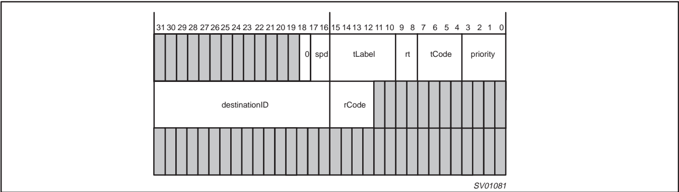
Figure 15. Quadlet/Block Write Response Packet Transmit Format
