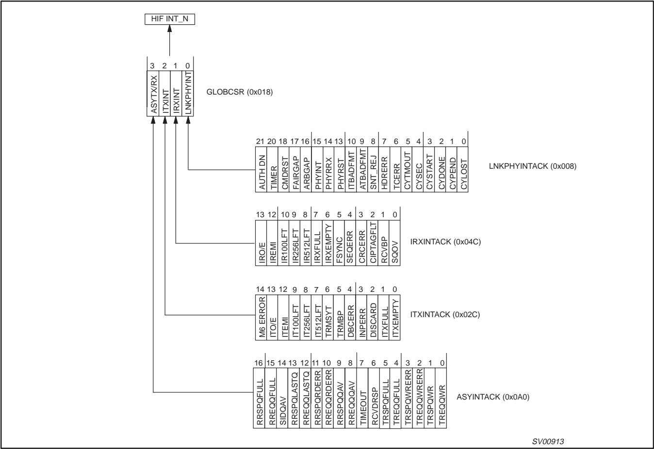
Figure 33. Interrupt Hierarchy
