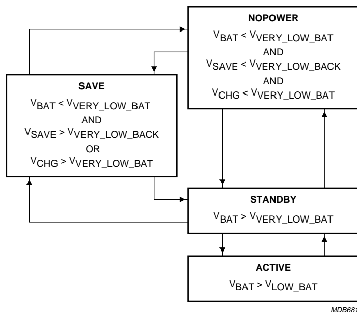
Fig.3 State diagram.
