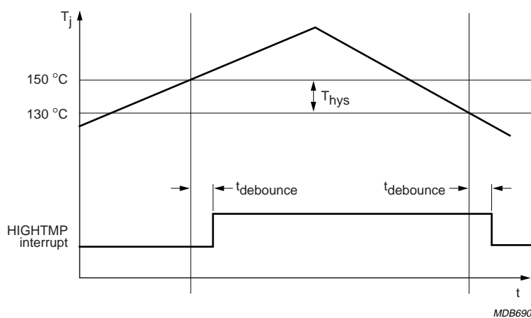
Fig.13 TS behaviour.
