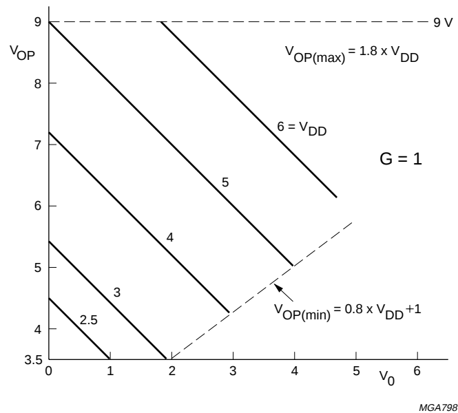
a. High-voltage mode V_{OP} = 1.8V_{DD} - V_0 .
