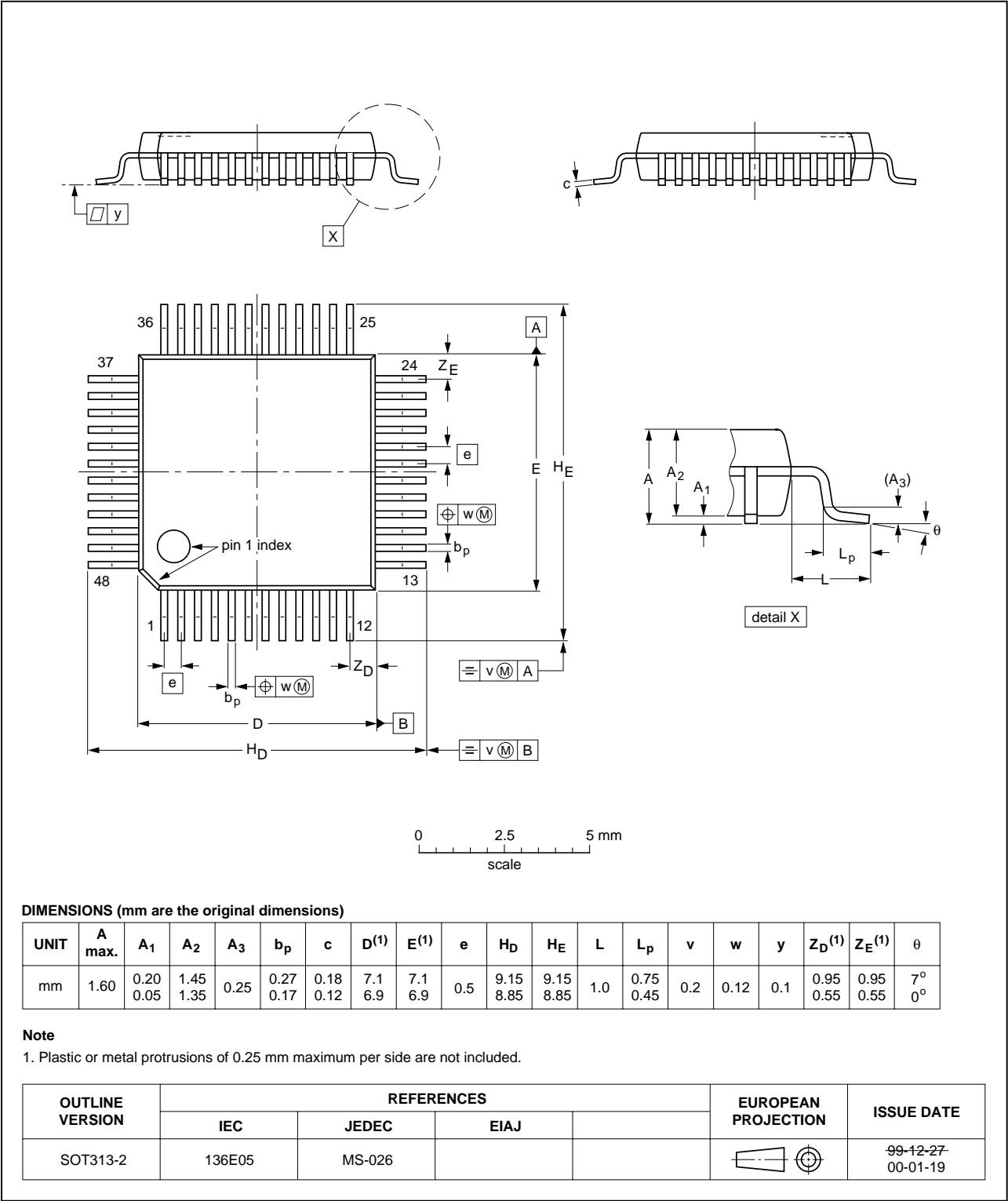
Fig 34. Package outline.
