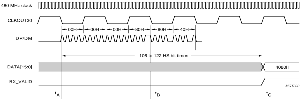
Fig 20. HS receive path delay.
