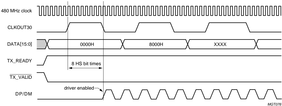
Fig 19. HS transmit path delay.
