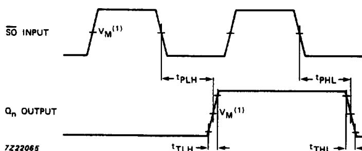
Fig.14 Waveforms showing \overline{SO} input to Q_n output propagation delays and output transition time.
