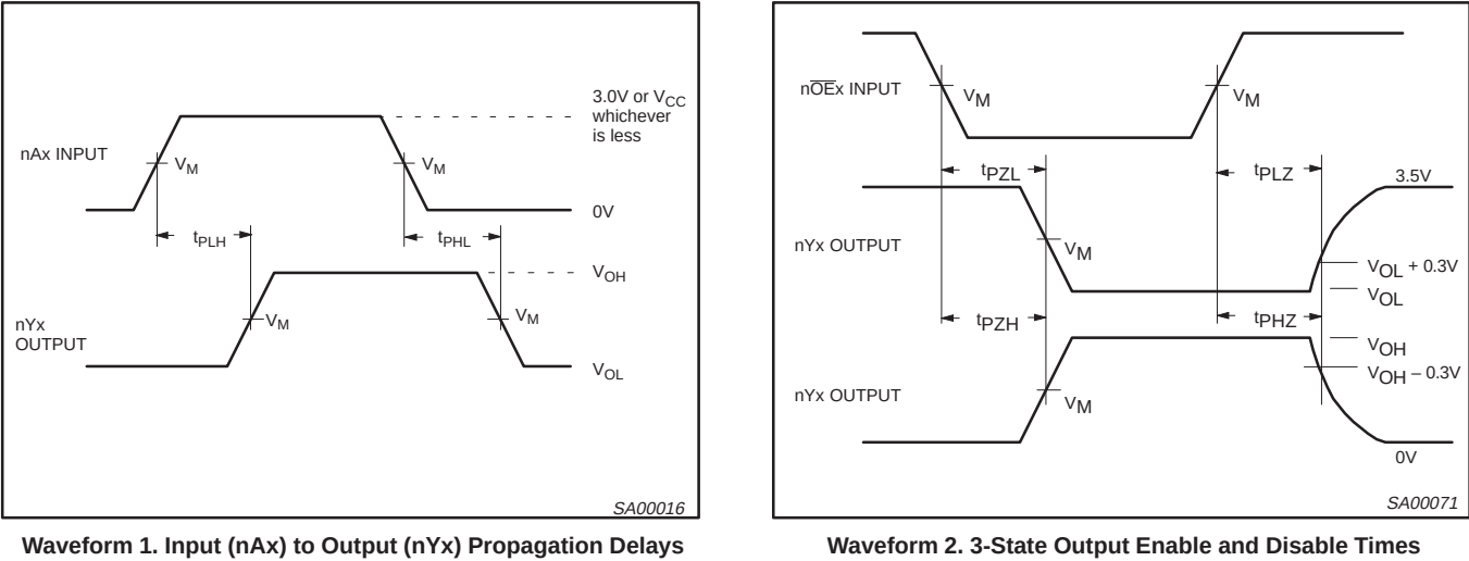
Waveform 1. Input (nAx) to Output (nYx) Propagation Delays
