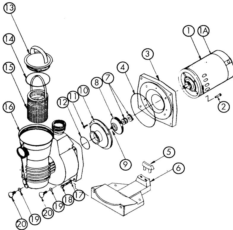
DRAWING NO. 34-9045
