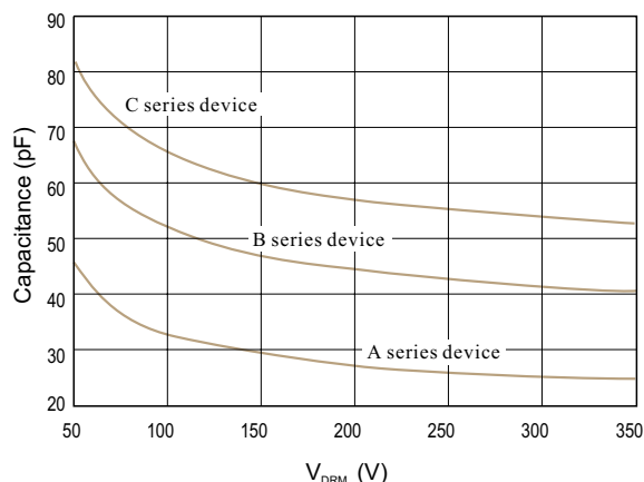
TYPICAL CAPACITANCE V.S. RATED REPETITIVE OFF-STATE VOLTAGE
