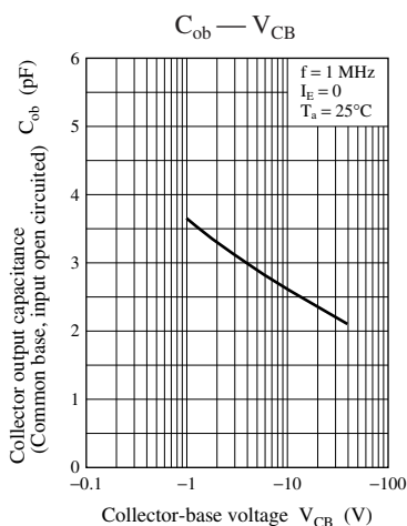
Characteristics charts of UNR1118
