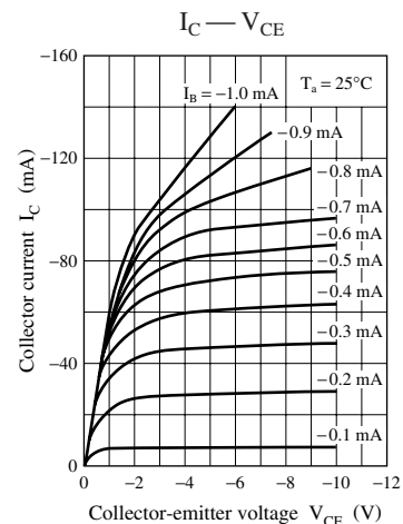
Characteristics charts of UNR1111
