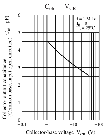
Characteristics charts of UNR1112
