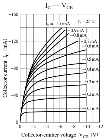
Characteristics charts of UNR1112
