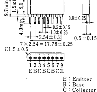
8-Lead Plastic SIL Package
