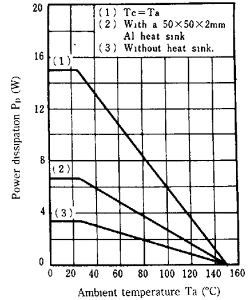
P_D - T_a (PU4219, PU4519)
